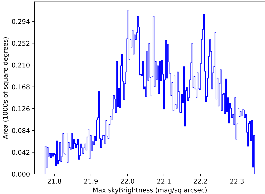
too_elab_r16_d2_giz_v3.4_10yrs Yr 1 g band: Max skyBrightness
