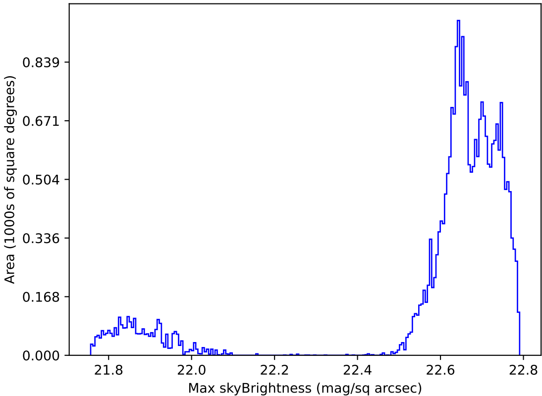
too_elab_r16_d2_giz_v3.4_10yrs Yr 1 all bands: Max skyBrightness
