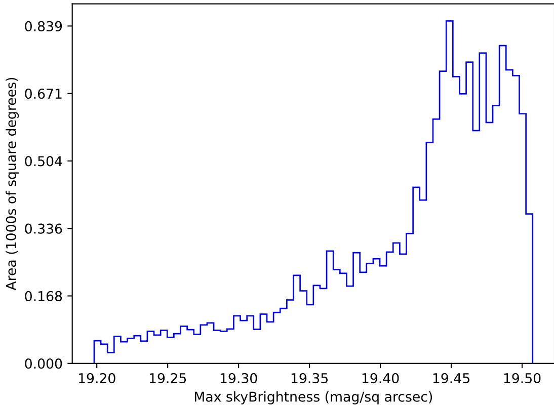
too_elab_r16_d2_giz_v3.4_10yrs WFD z band: Max skyBrightness
