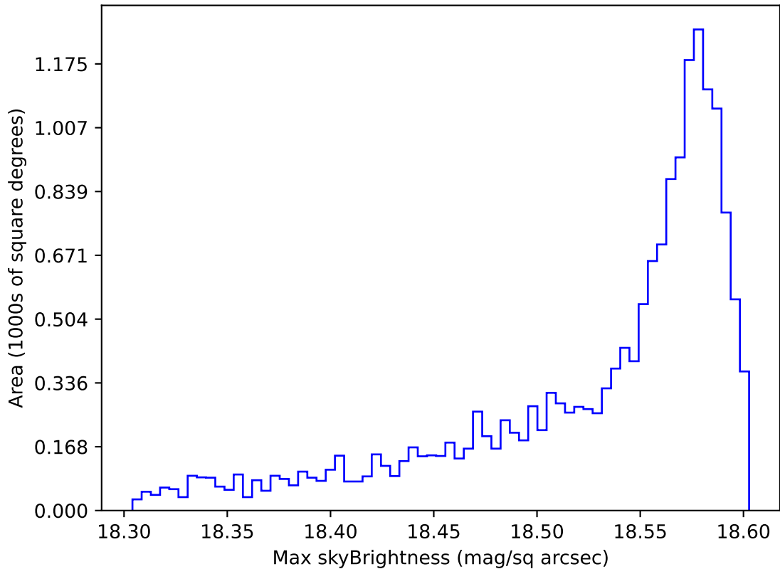
too_elab_r16_d2_giz_v3.4_10yrs WFD y band: Max skyBrightness
