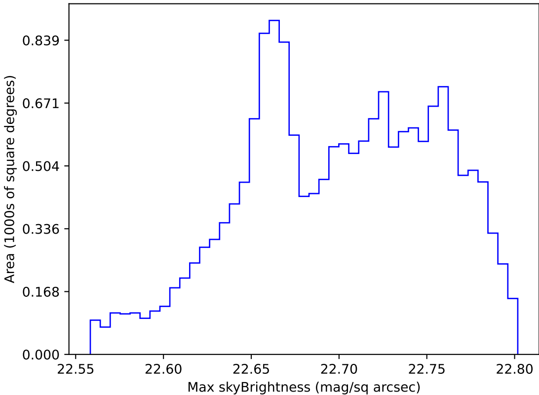
too_elab_r16_d2_giz_v3.4_10yrs WFD u band: Max skyBrightness
