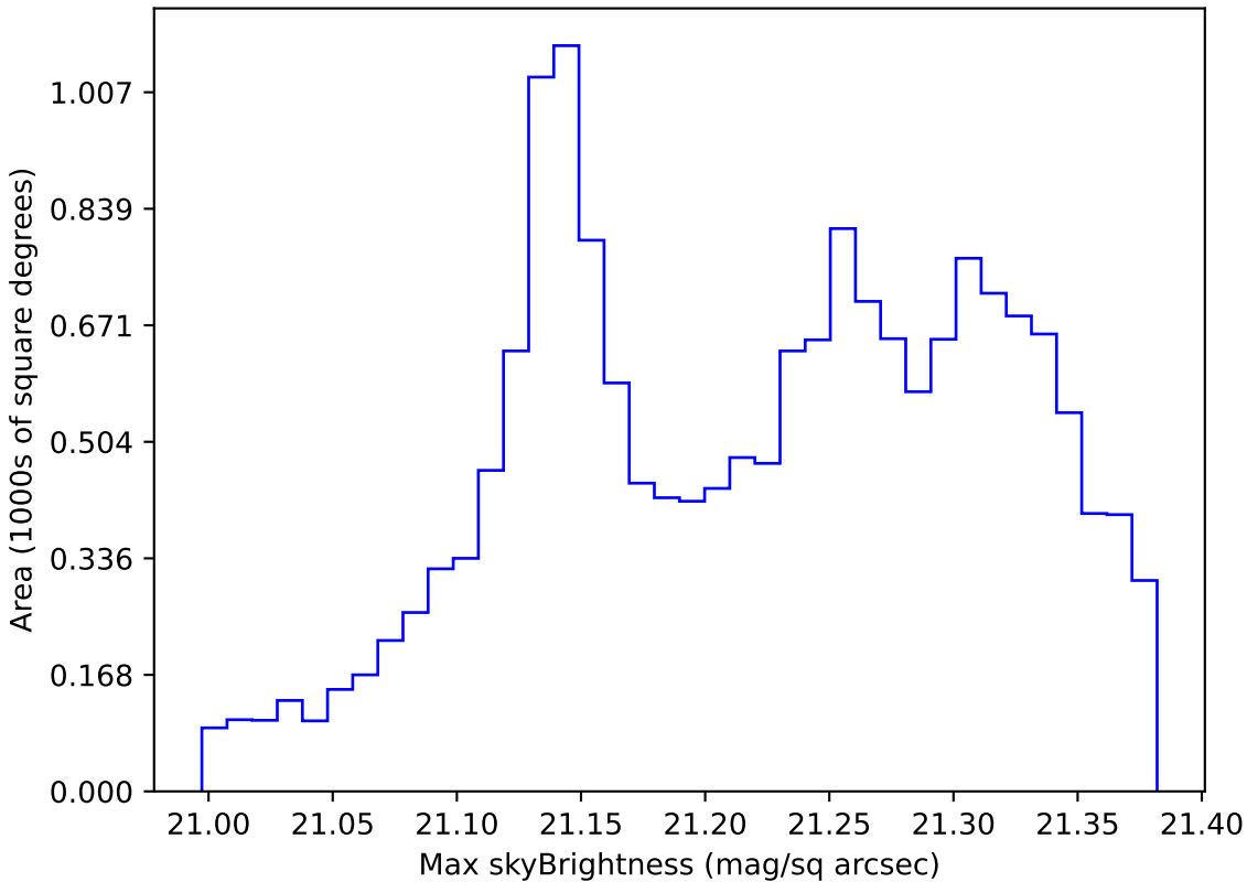
too_elab_r16_d2_giz_v3.4_10yrs WFD r band: Max skyBrightness
