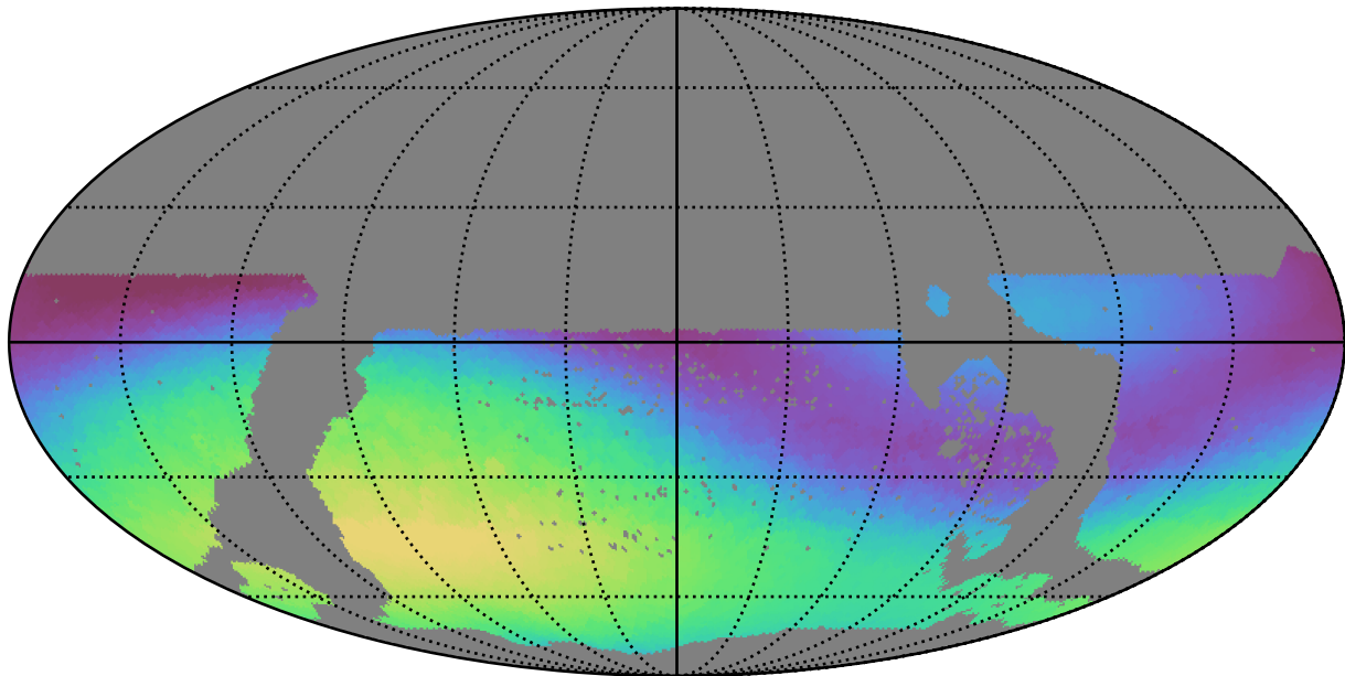
too_elab_r16_d2_giz_v3.4_10yrs WFD g band: Max skyBrightness
