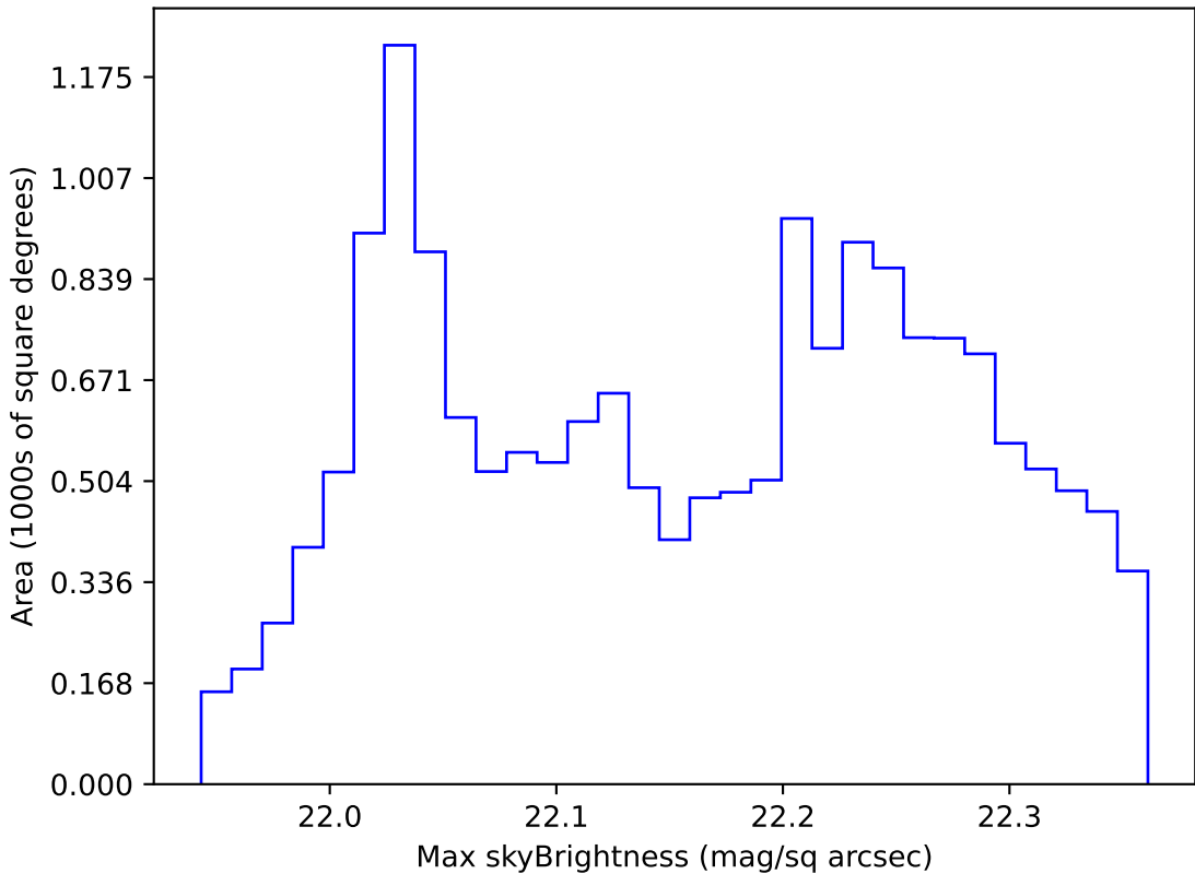
too_elab_r16_d2_giz_v3.4_10yrs WFD g band: Max skyBrightness
