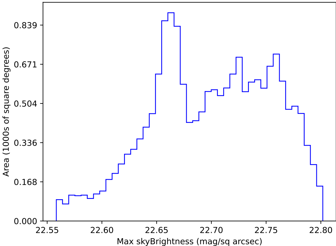
too_elab_r16_d2_giz_v3.4_10yrs WFD all bands: Max skyBrightness
