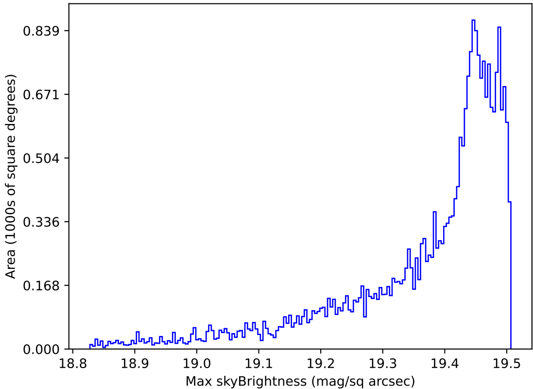
too_elab_r16_d2_giz_v3.4_10yrs All sky z band: Max skyBrightness
