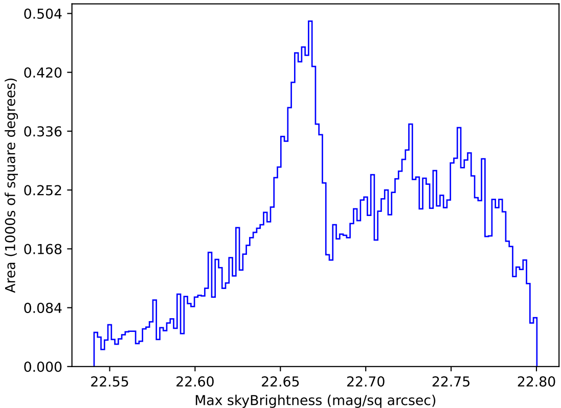
too_elab_r16_d2_giz_v3.4_10yrs All sky u band: Max skyBrightness
