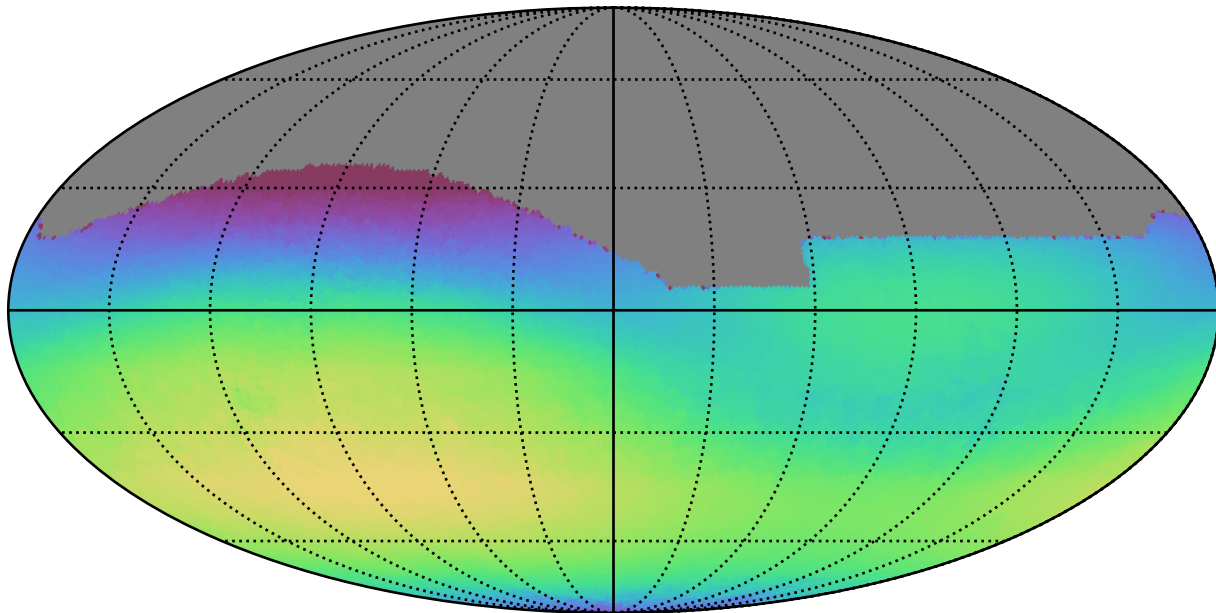
too_elab_r16_d2_giz_v3.4_10yrs All sky r band: Max skyBrightness
