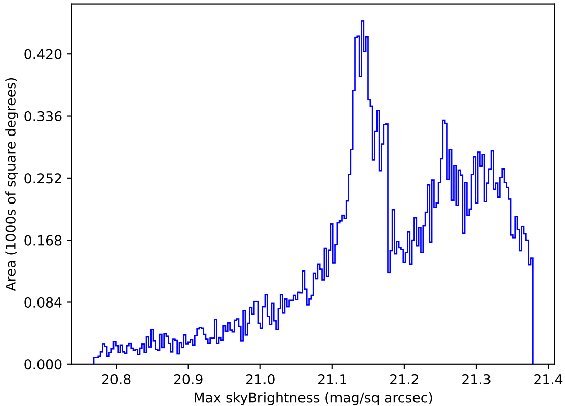
too_elab_r16_d2_giz_v3.4_10yrs All sky r band: Max skyBrightness
