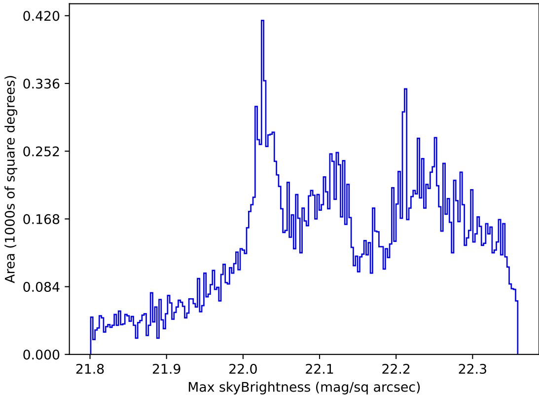
too_elab_r16_d2_giz_v3.4_10yrs All sky g band: Max skyBrightness
