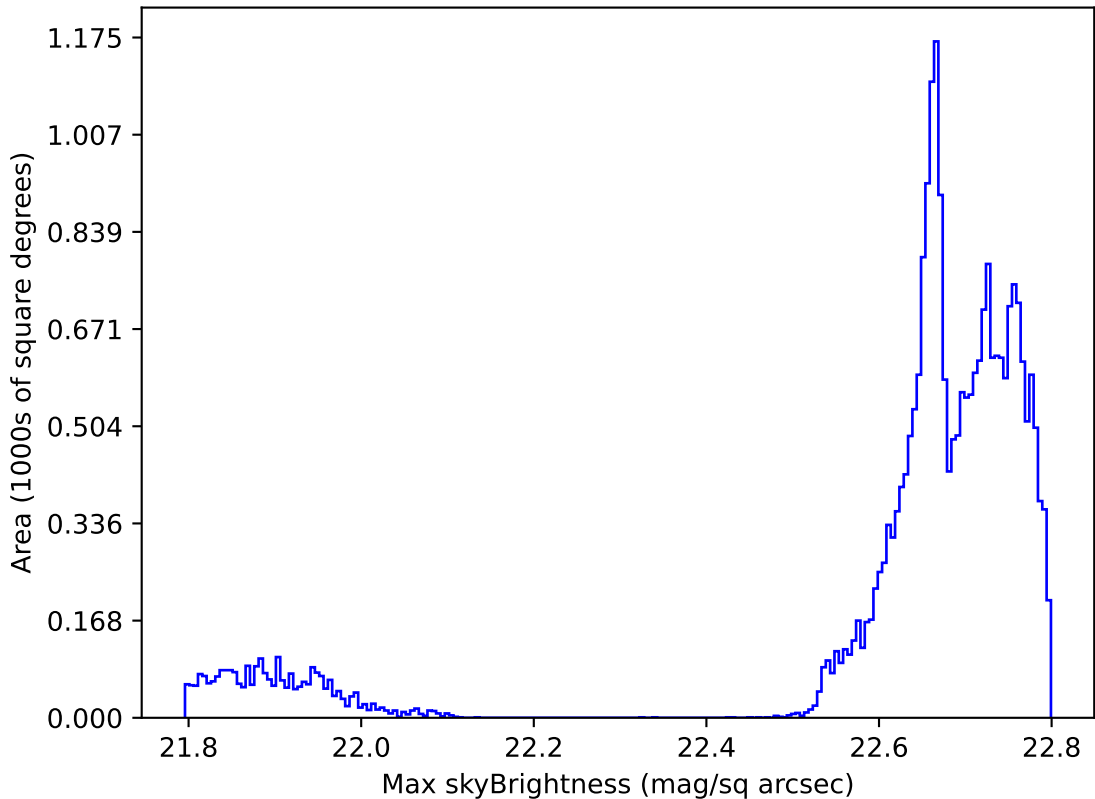
too_elab_r16_d2_giz_v3.4_10yrs All sky all bands: Max skyBrightness
