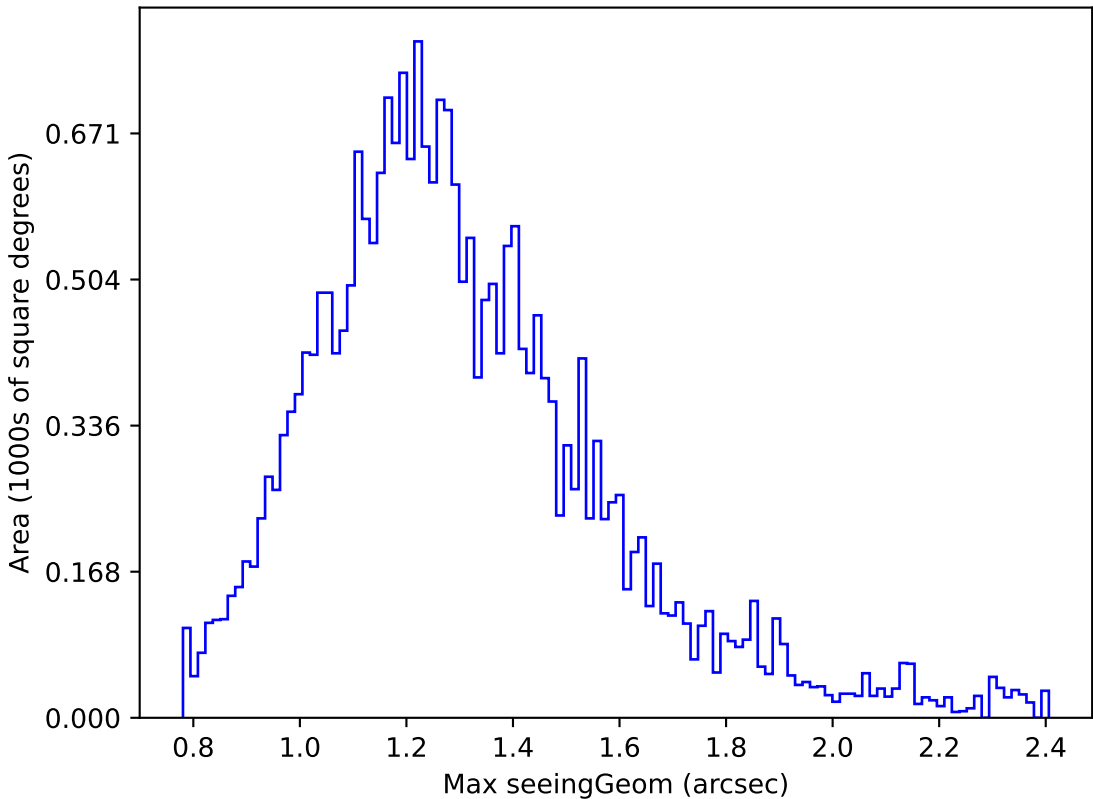
too_elab_r16_d2_giz_v3.4_10yrs Yr 1 z band: Max seeingGeom
