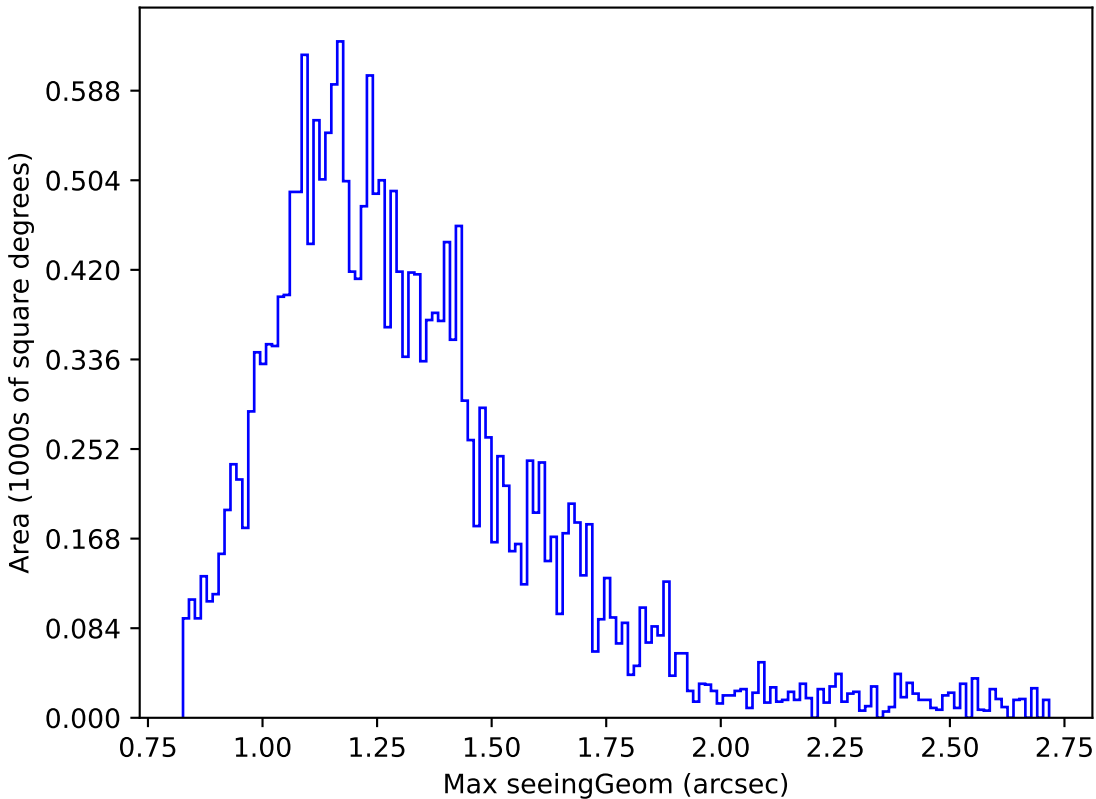
too_elab_r16_d2_giz_v3.4_10yrs Yr 1 u band: Max seeingGeom
