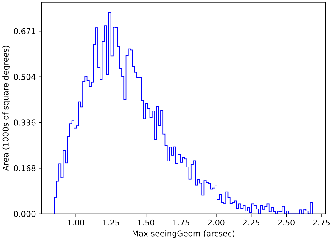
too_elab_r16_d2_giz_v3.4_10yrs Yr 1 r band: Max seeingGeom
