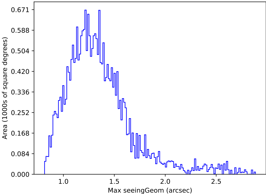
too_elab_r16_d2_giz_v3.4_10yrs Yr 1 i band: Max seeingGeom
