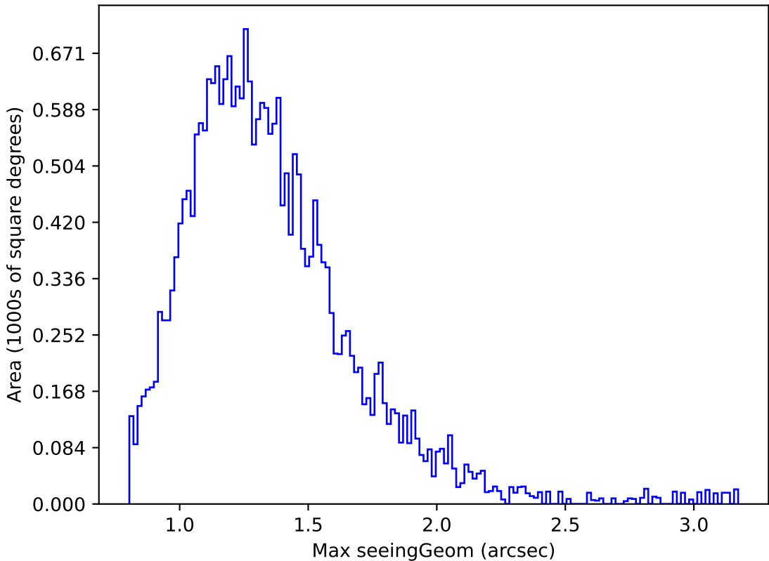
too_elab_r16_d2_giz_v3.4_10yrs Yr 1 g band: Max seeingGeom
