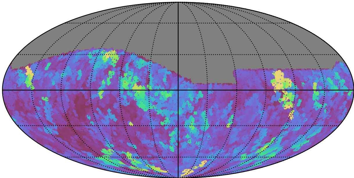
too_elab_r16_d2_giz_v3.4_10yrs Yr 1 all bands: Max seeingEff
