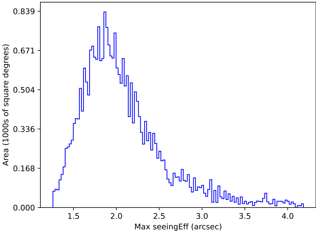
too_elab_r16_d2_giz_v3.4_10yrs Yr 1 all bands: Max seeingEff
