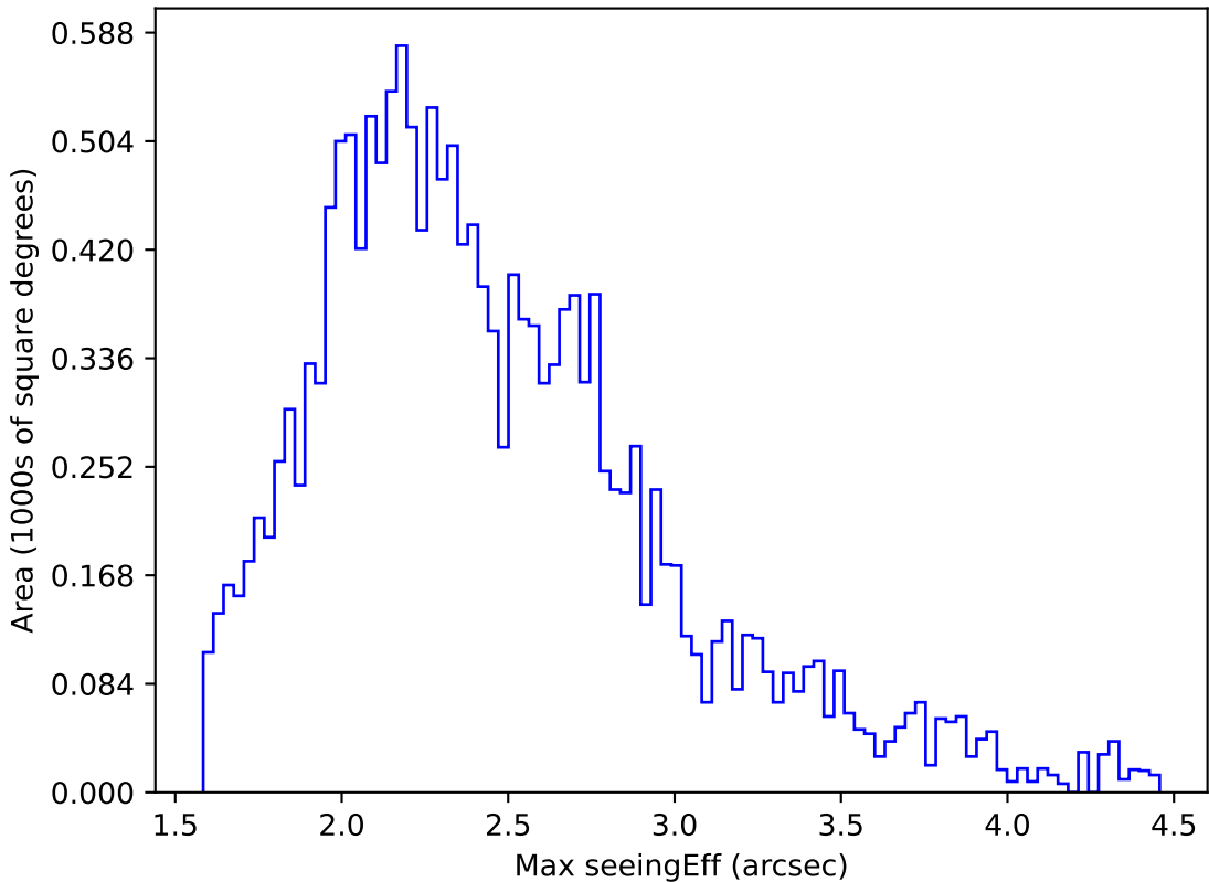
too_elab_r16_d2_giz_v3.4_10yrs WFD y band: Max seeingEff
