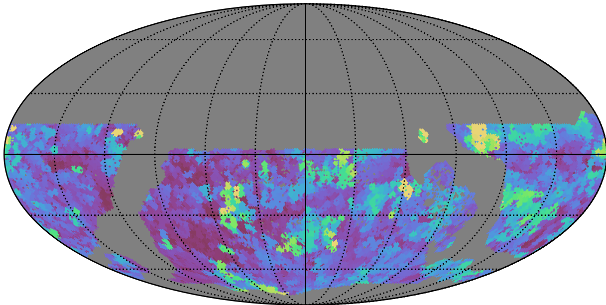
too_elab_r16_d2_giz_v3.4_10yrs WFD g band: Max seeingEff
