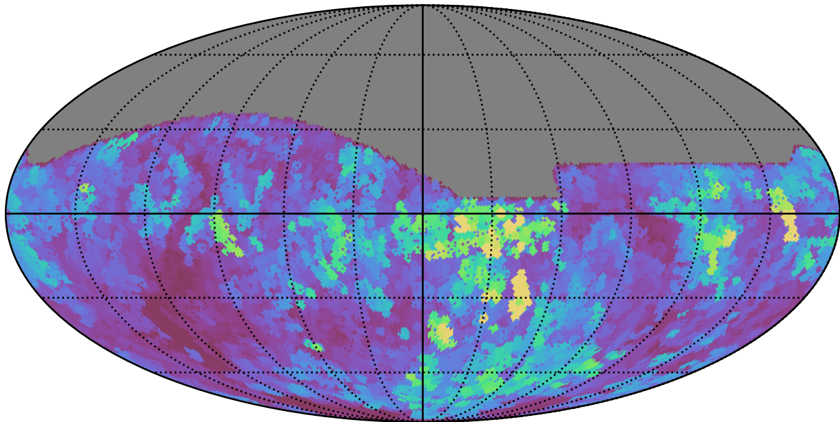
too_elab_r16_d2_giz_v3.4_10yrs All sky z band: Max seeingEff
