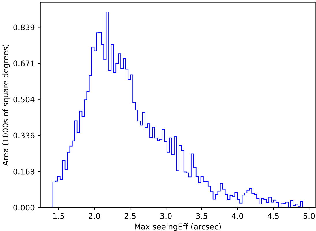
too_elab_r16_d2_giz_v3.4_10yrs All sky z band: Max seeingEff
