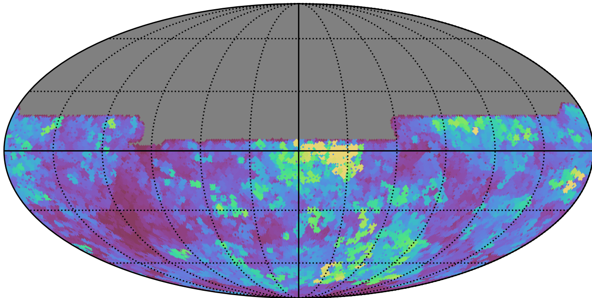
too_elab_r16_d2_giz_v3.4_10yrs All sky y band: Max seeingEff
