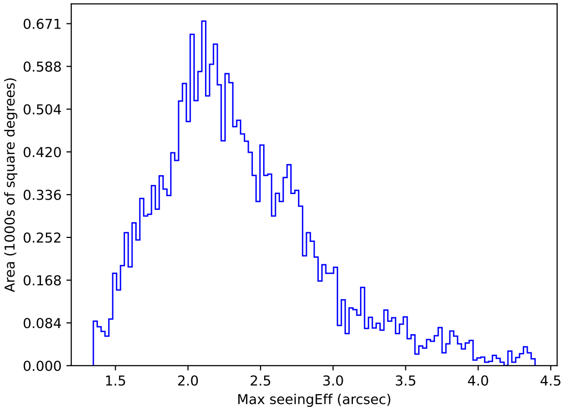
too_elab_r16_d2_giz_v3.4_10yrs All sky y band: Max seeingEff
