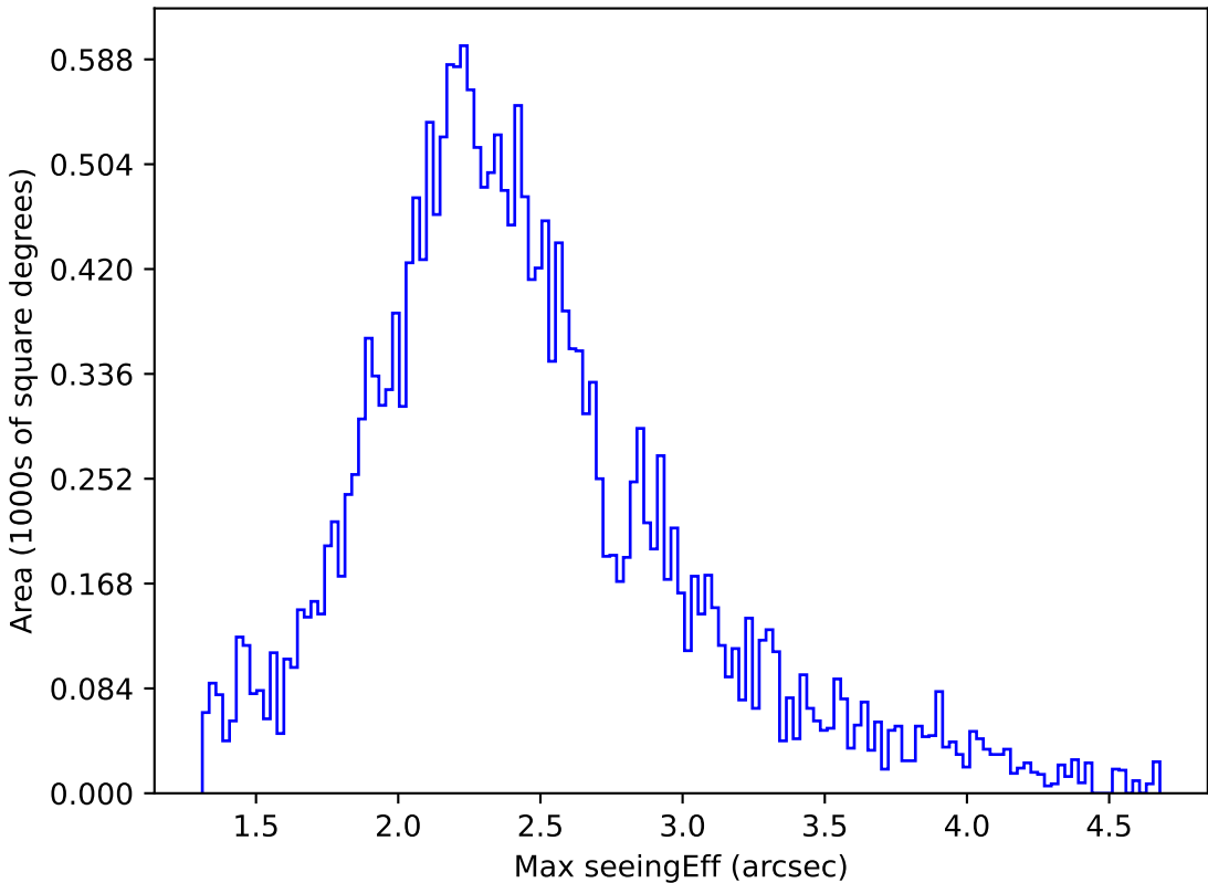
too_elab_r16_d2_giz_v3.4_10yrs All sky u band: Max seeingEff
