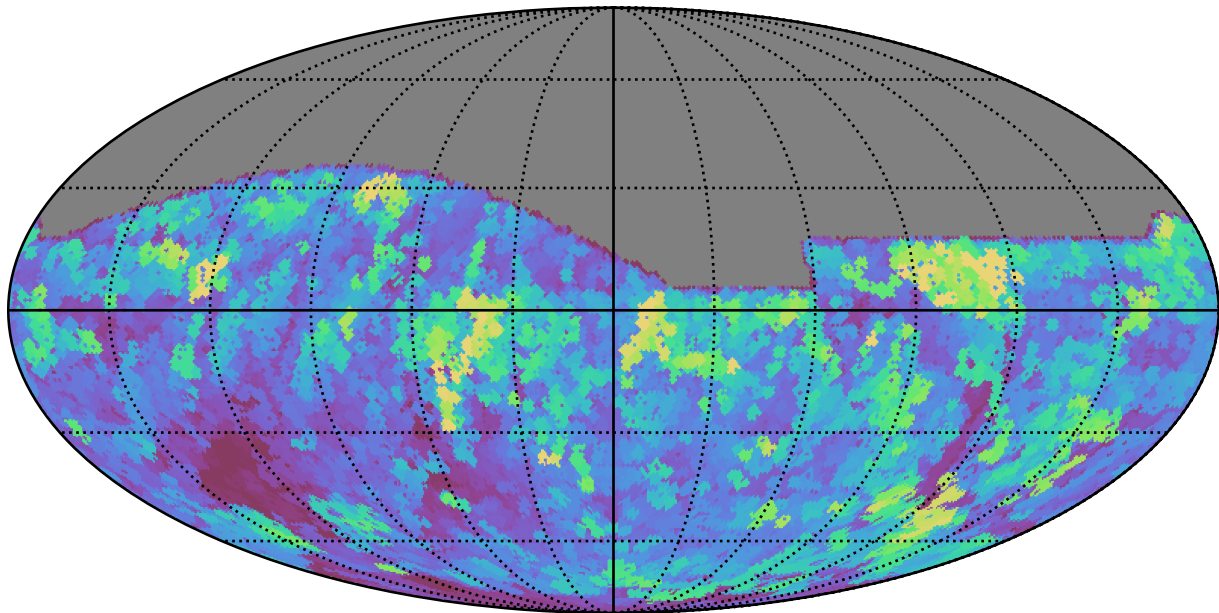
too_elab_r16_d2_giz_v3.4_10yrs All sky r band: Max seeingEff
