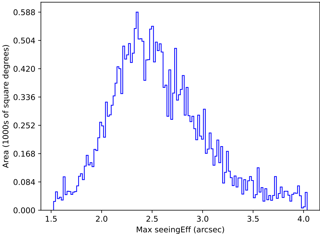
too_elab_r16_d2_giz_v3.4_10yrs All sky r band: Max seeingEff
