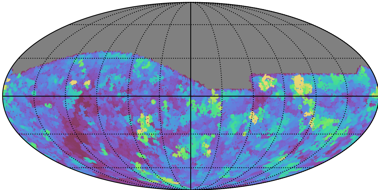
too_elab_r16_d2_giz_v3.4_10yrs All sky g band: Max seeingEff
