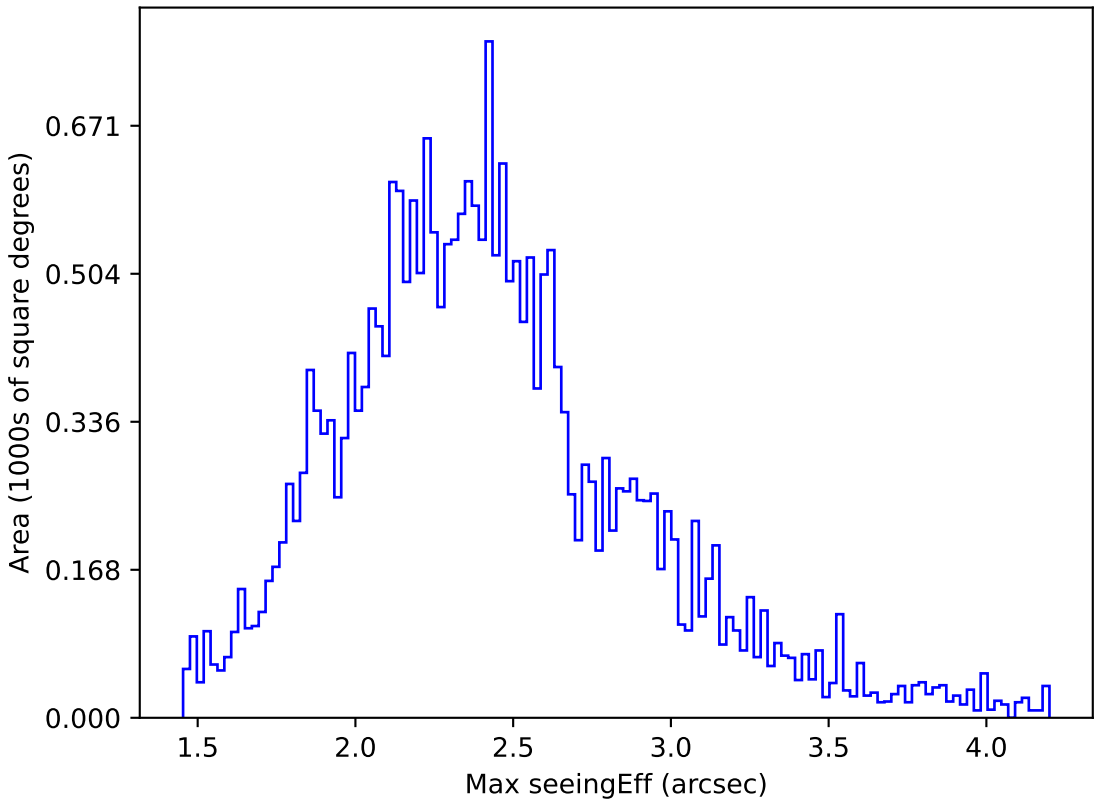
too_elab_r16_d2_giz_v3.4_10yrs All sky g band: Max seeingEff
