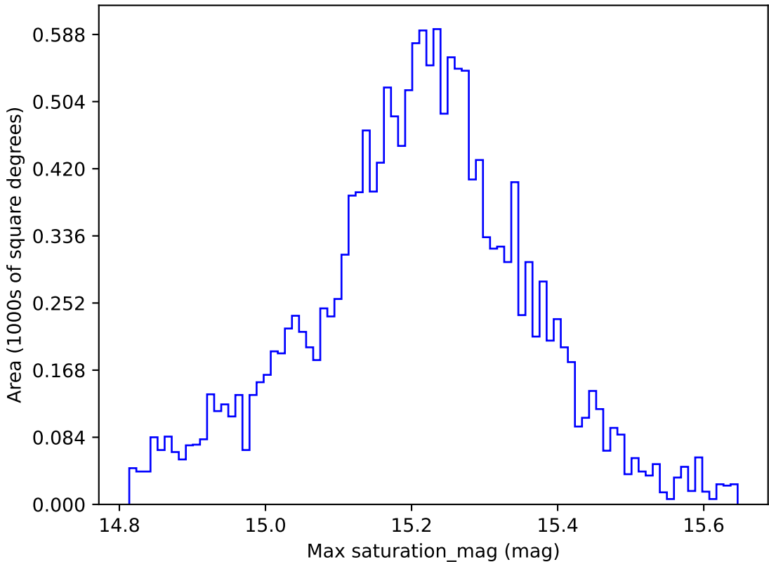
too_elab_r16_d2_giz_v3.4_10yrs WFD z band: Max saturation_mag
