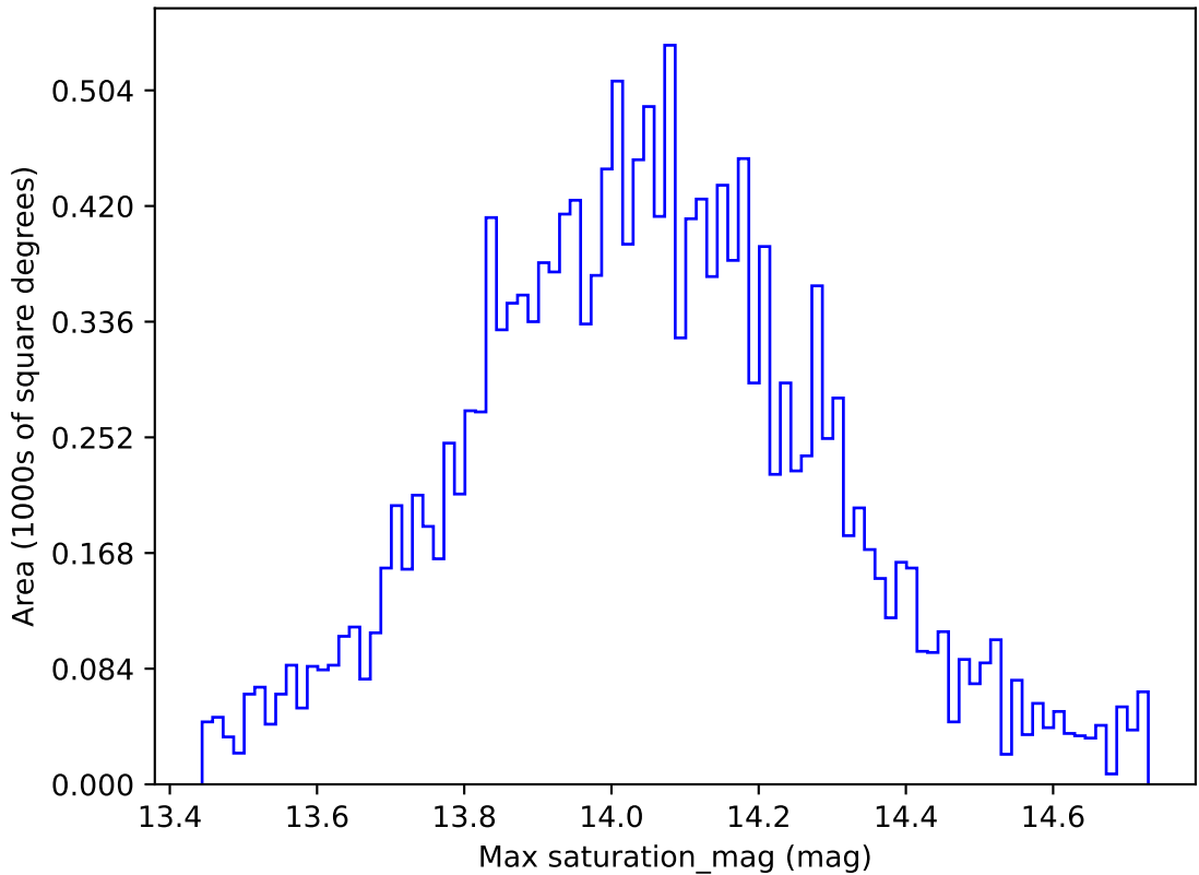
too_elab_r16_d2_giz_v3.4_10yrs WFD u band: Max saturation_mag
