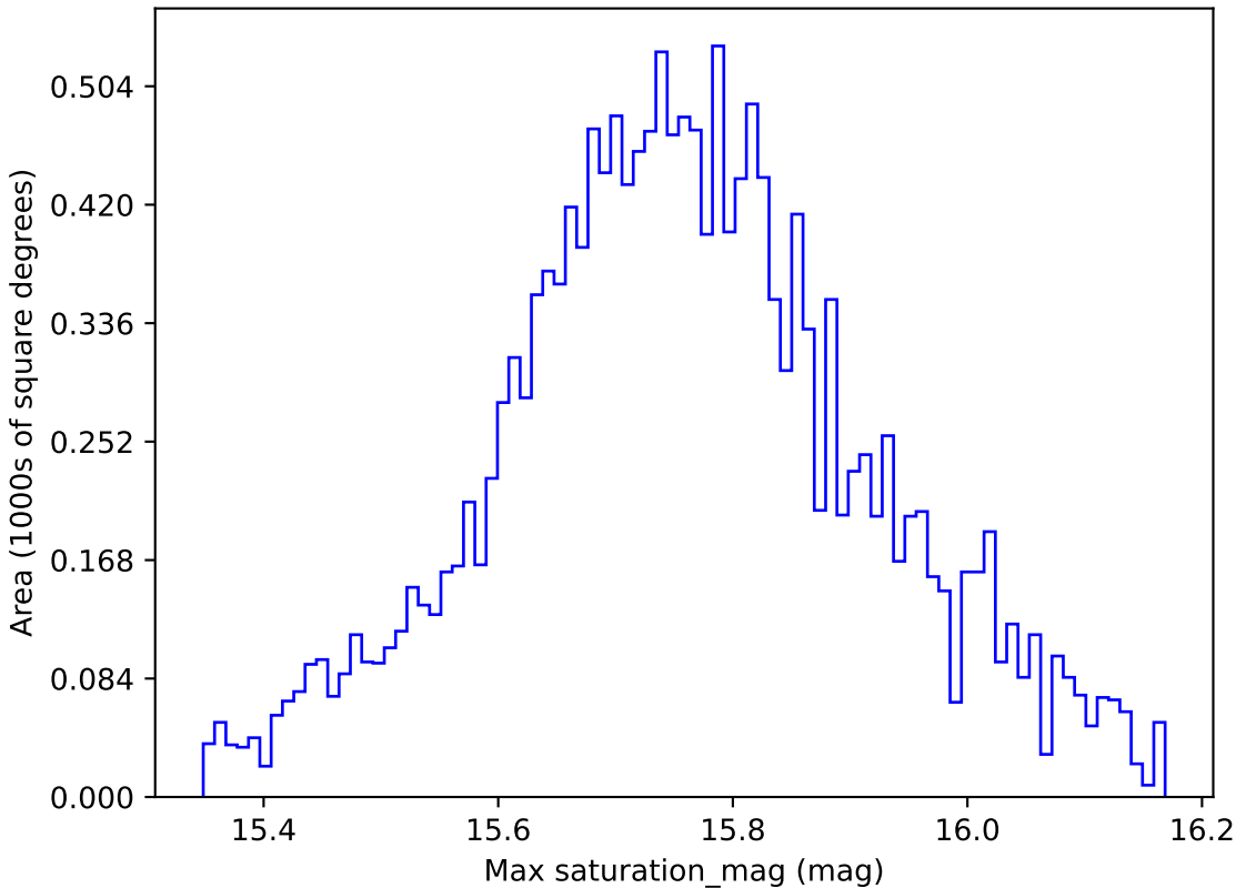
too_elab_r16_d2_giz_v3.4_10yrs WFD r band: Max saturation_mag
