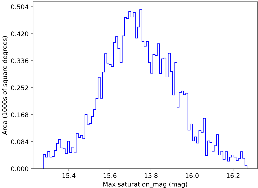
too_elab_r16_d2_giz_v3.4_10yrs WFD g band: Max saturation_mag
