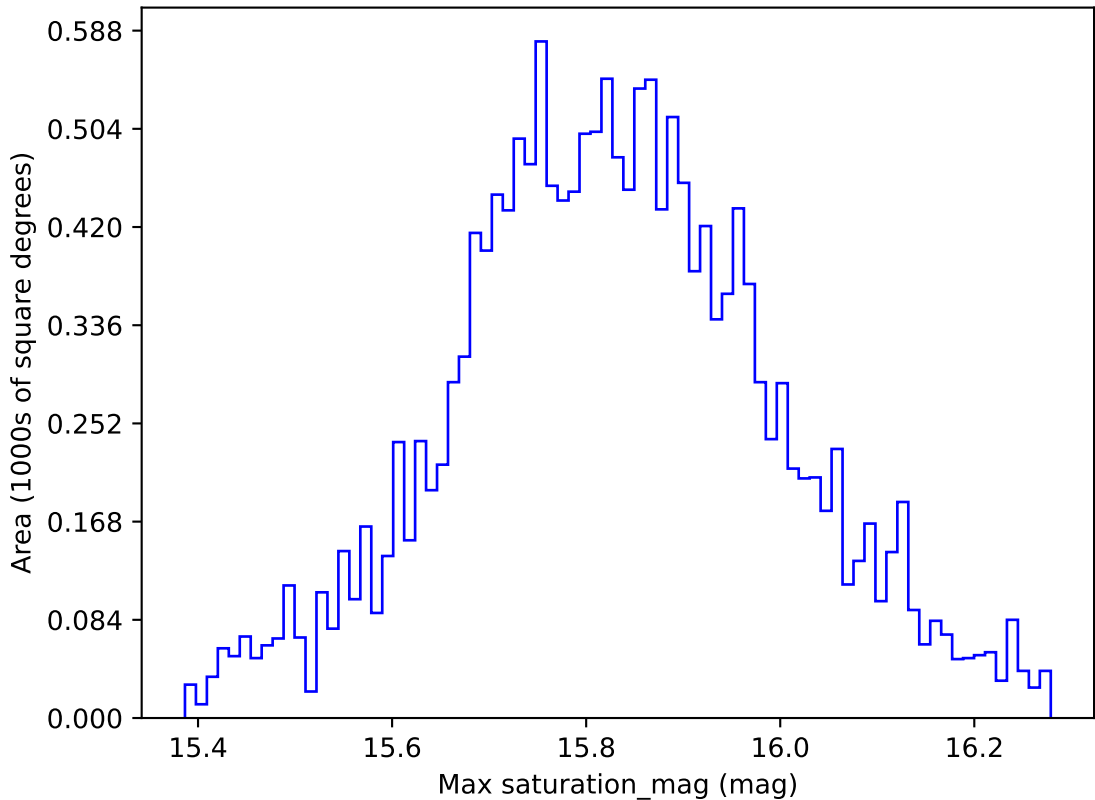
too_elab_r16_d2_giz_v3.4_10yrs WFD all bands: Max saturation_mag
