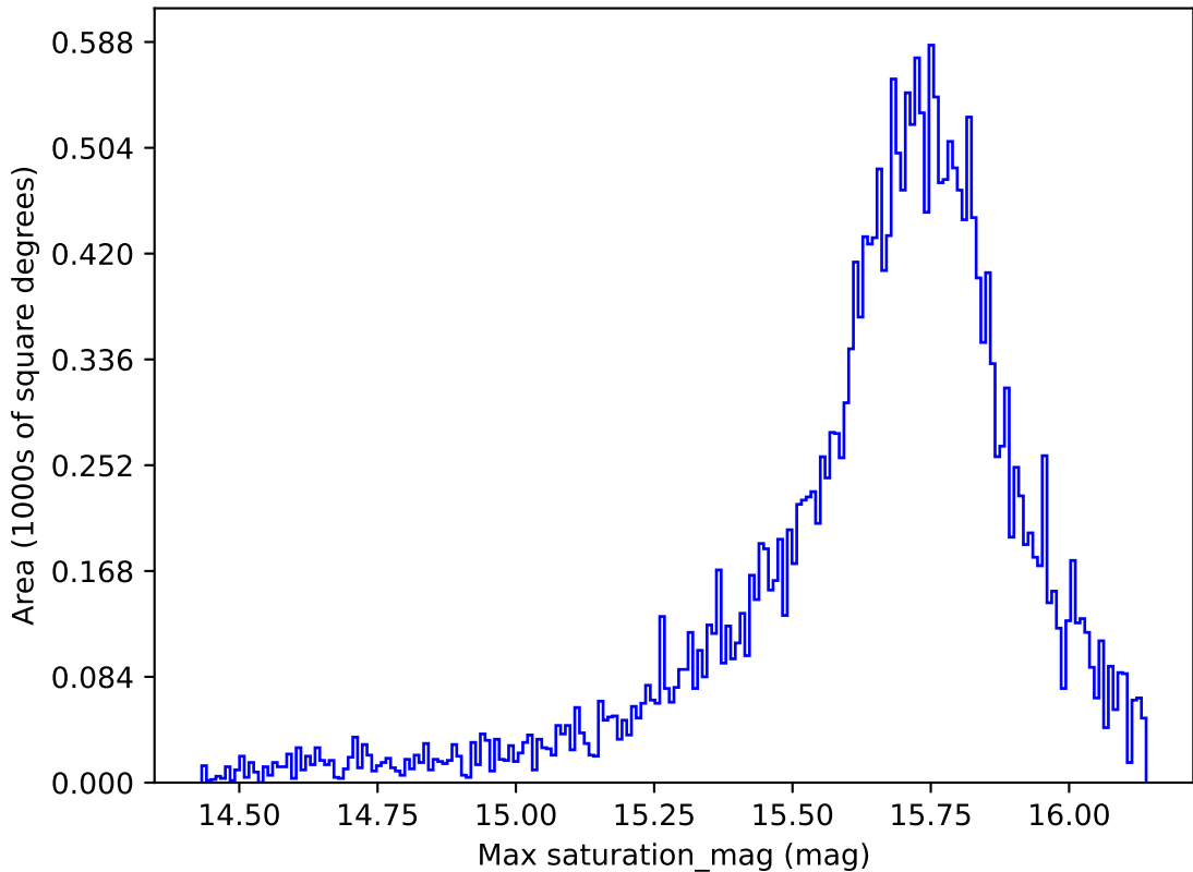
too_elab_r16_d2_giz_v3.4_10yrs All sky r band: Max saturation_mag
