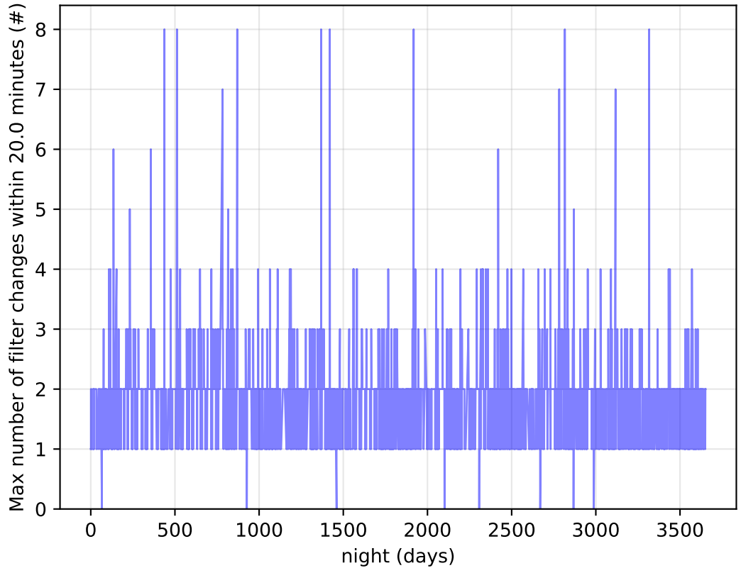
too_elab_r16_d2_giz_v3.4_10yrs Per Night: Max number of filter changes within 20.0 minutes
