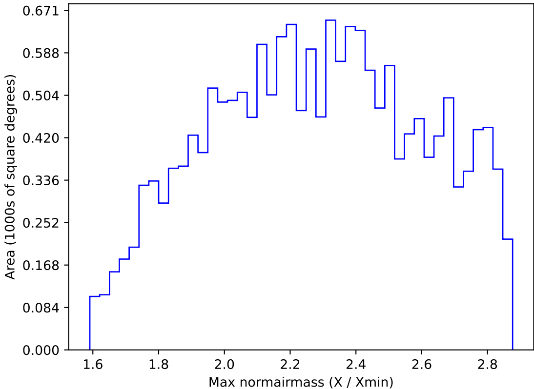
too_elab_r16_d2_giz_v3.4_10yrs WFD z band: Max normairmass
