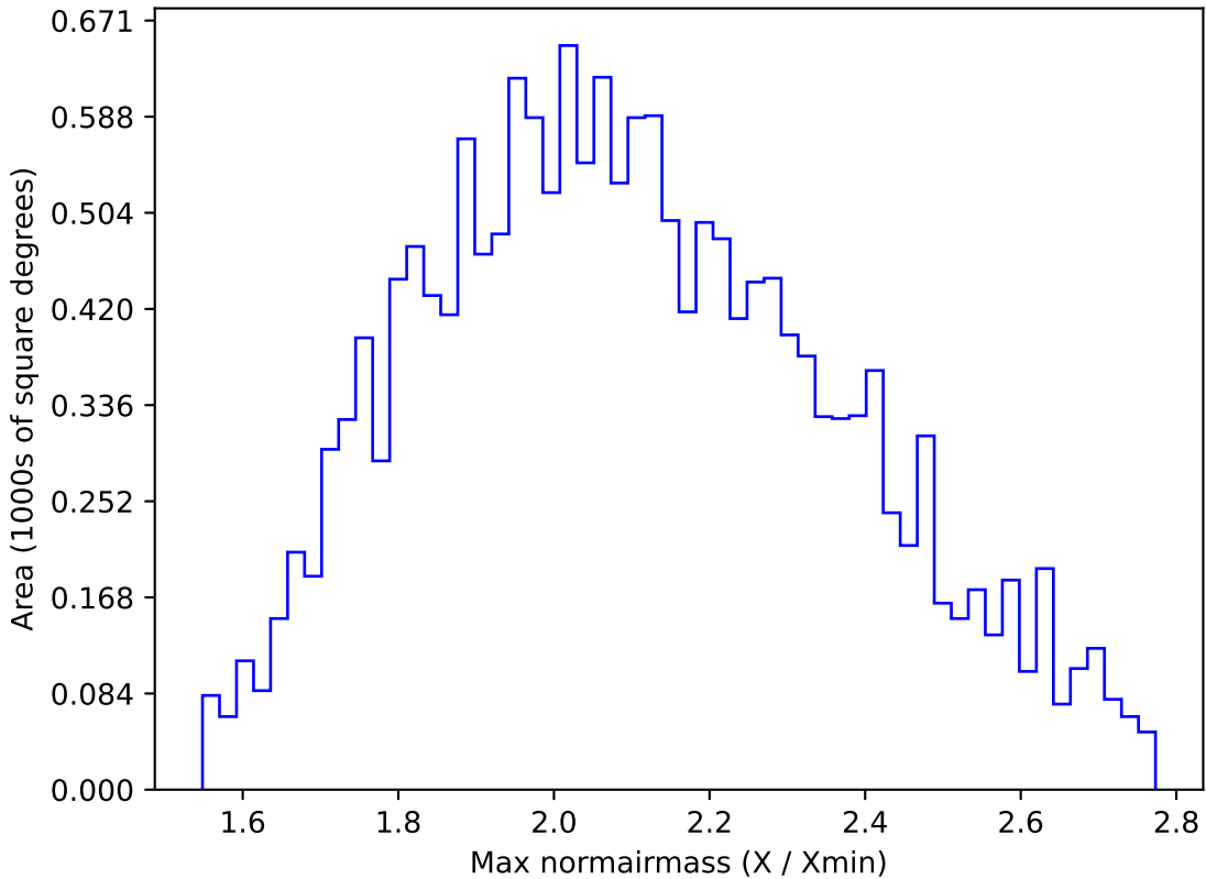
too_elab_r16_d2_giz_v3.4_10yrs WFD y band: Max normairmass
