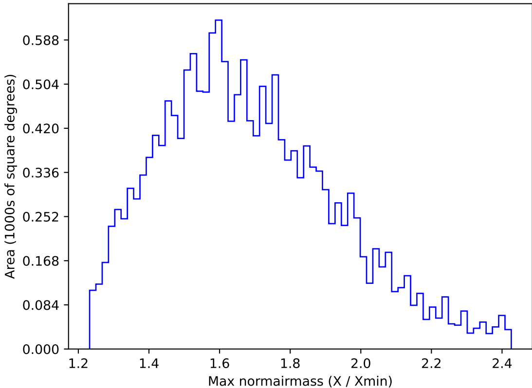
too_elab_r16_d2_giz_v3.4_10yrs WFD u band: Max normairmass
