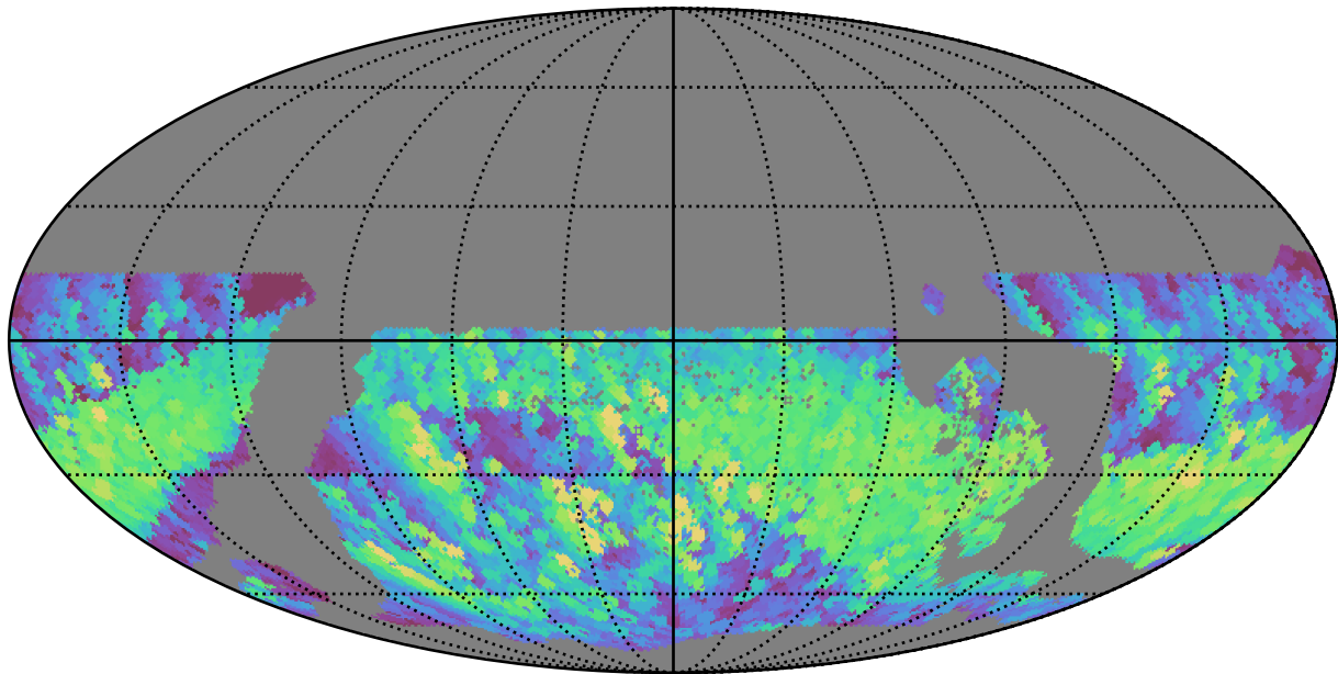
too_elab_r16_d2_giz_v3.4_10yrs WFD r band: Max normairmass
