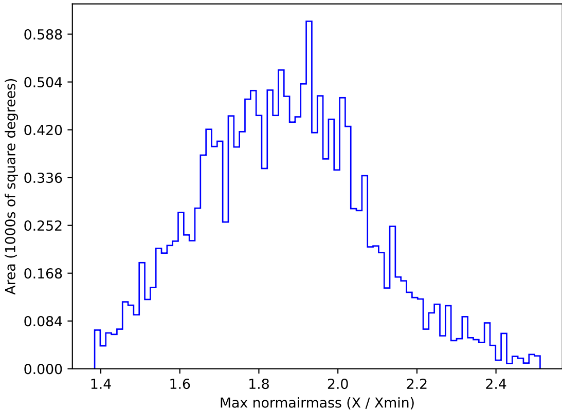
too_elab_r16_d2_giz_v3.4_10yrs WFD g band: Max normairmass
