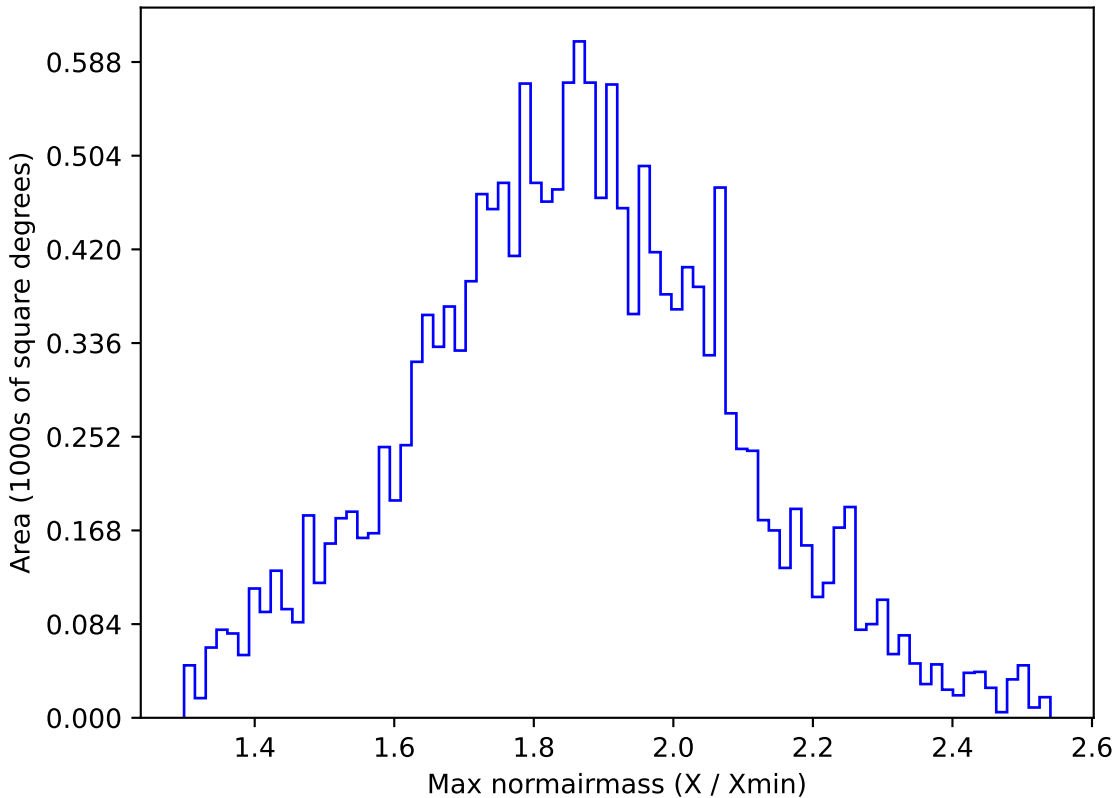
too_elab_r16_d2_giz_v3.4_10yrs WFD g band: Max normairmass
