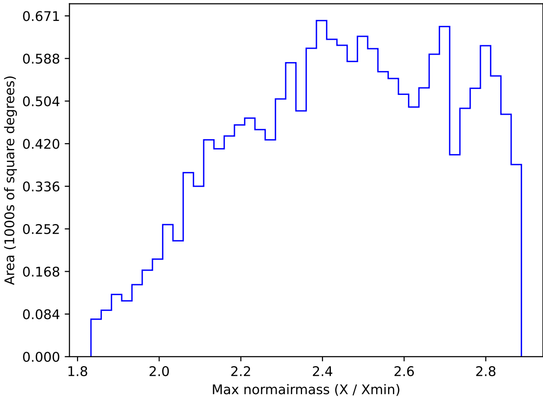
too_elab_r16_d2_giz_v3.4_10yrs WFD all bands: Max normairmass
