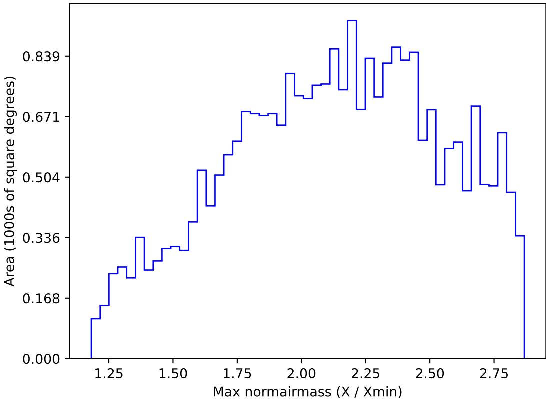
too_elab_r16_d2_giz_v3.4_10yrs All sky z band: Max normairmass
