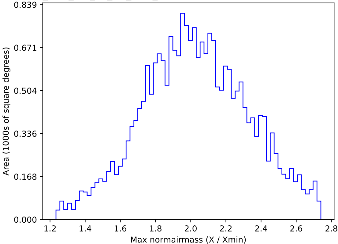
too_elab_r16_d2_giz_v3.4_10yrs All sky y band: Max normairmass
