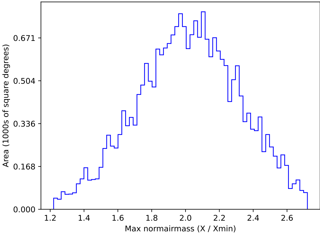
too_elab_r16_d2_giz_v3.4_10yrs All sky y band: Max normairmass
