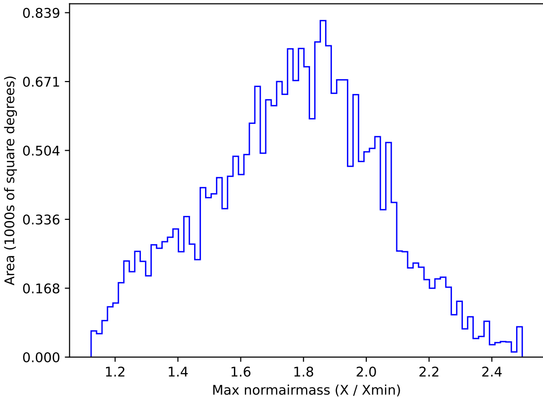
too_elab_r16_d2_giz_v3.4_10yrs All sky g band: Max normairmass
