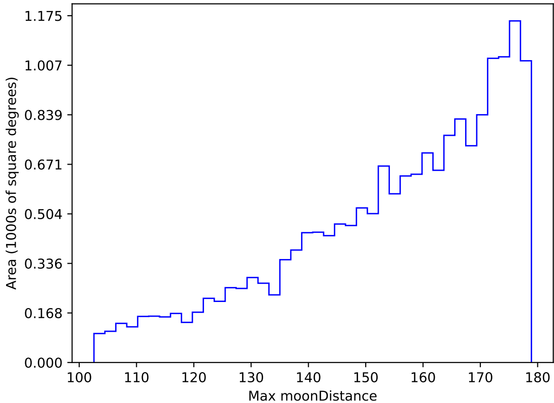
too_elab_r16_d2_giz_v3.4_10yrs WFD z band: Max moonDistance
